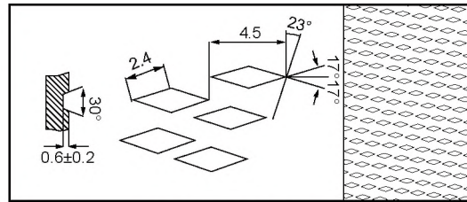
Inside Dia. > 22
